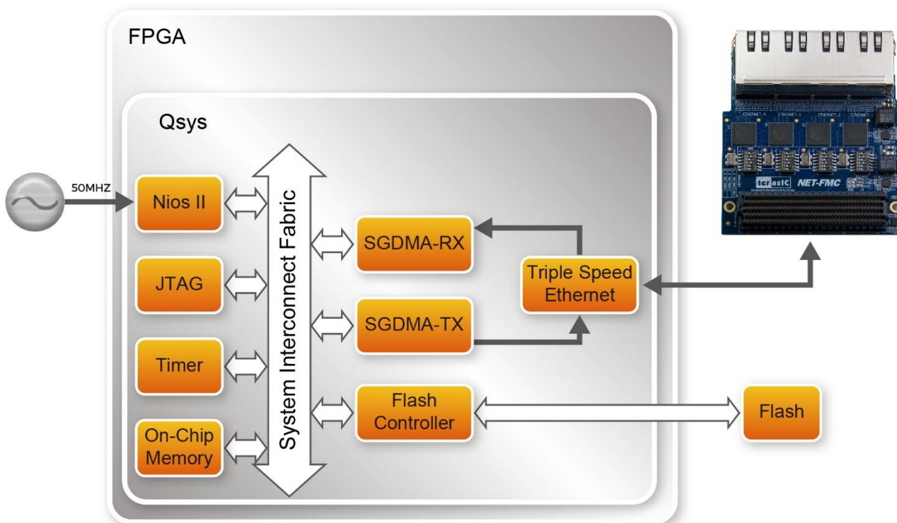
Figure 4-2 Function block diagram of remote-update portal demonstration
